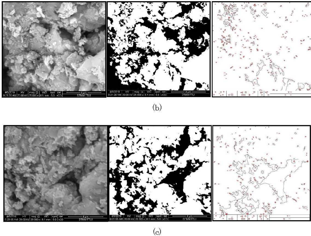
Fig. 8. SEM Testing Results at Magnification 25000x (a) SPP320, (b) SPP360, (c) SPP400
