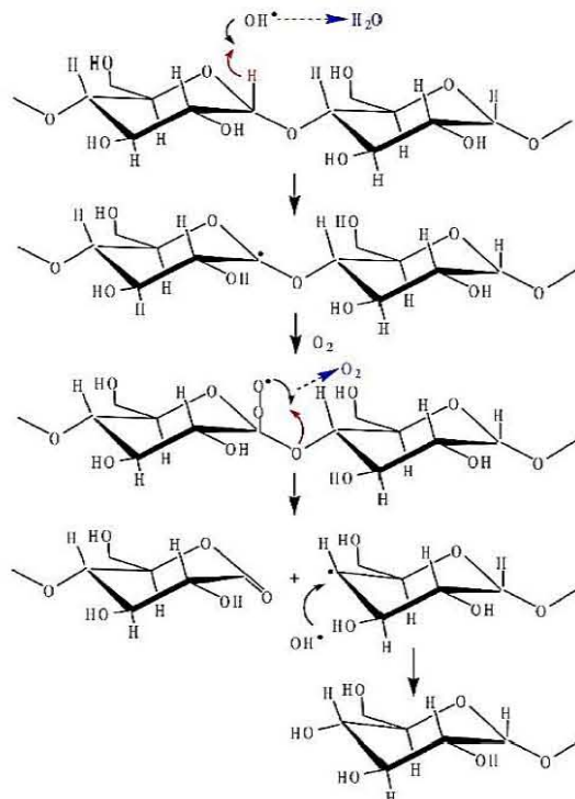
Fig. 4. Scheme Degradation of Glycosidic bond by oxygen radical species ( \text{OH}^* ) [25].
