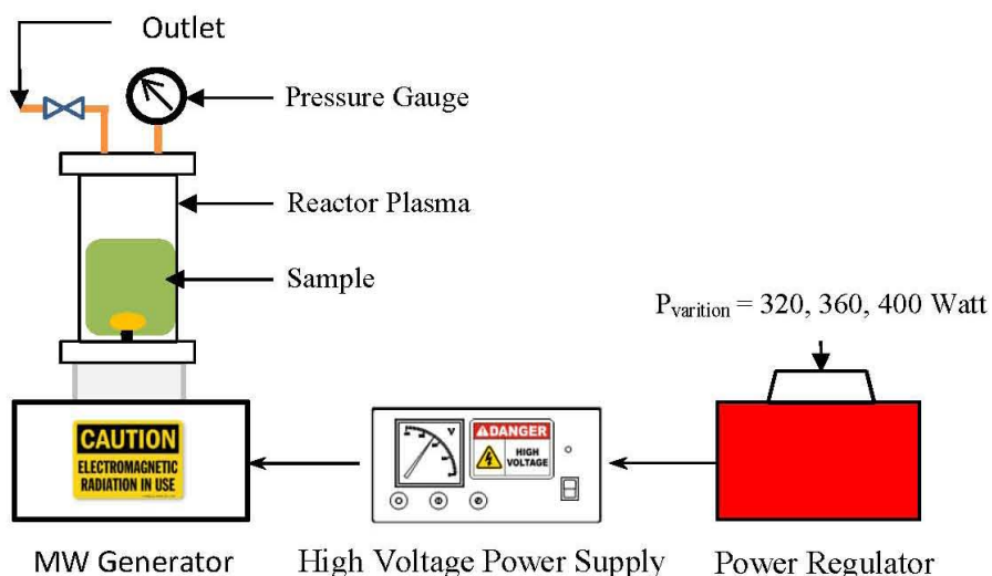
Fig. 2. The Schematic Apparatus of PT in-Water
